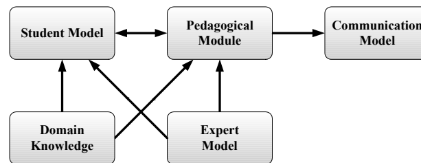
Figure 1: Main Components of Intelligent Learning Systems
