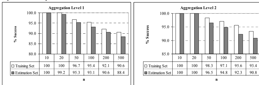
Figure 6: Average Experimental Results for Learning Objects
