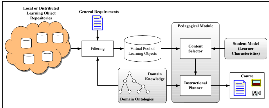
Figure 1: Generalized Framework of Automatic Course Sequencing
