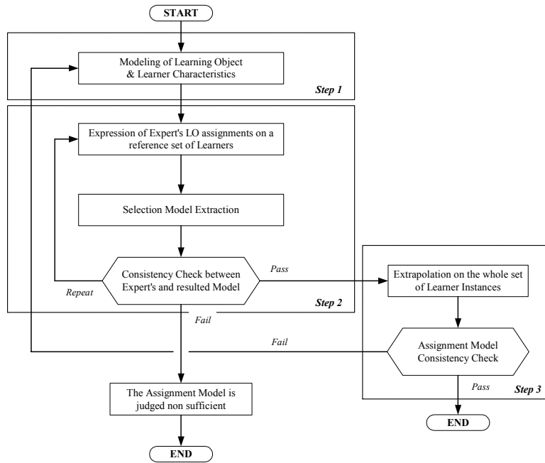
Figure 2: Selection Model Extraction Framework
