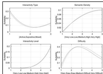
Figure 5: Marginal Suitability for a specific Learner (Continuous line represents the real expert's model and the dashed one the resulted approximation)
