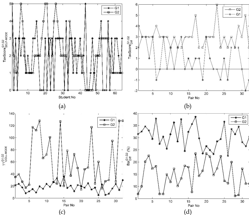
Figure 1. (a) The estimated \text{TaxScore}_{\text{SELF-MODE}}^{\text{G1,G2}} values across all students per group, (b) The \text{TaxScore}_{\text{Diff}}^{\text{G1,G2}} values across the pairs of both G1 and G2 groups, i.e., \text{TaxScore}_{\text{Diff}}^{\text{G1,G2}} (c) The \text{TT}_{\text{COLL-MODE}}^{\text{G1,G2}} values across the pairs of both G1 and G2 groups, i.e., \text{TT}_{\text{COLL-MODE}}^{\text{G1,G2}} , and (d) The \text{Bal}_{\text{Diff}}^{\text{G1,G2}} values across the pairs of both G1 and G2 groups, i.e., \text{Bal}_{\text{Diff}}^{\text{G1,G2}} .
